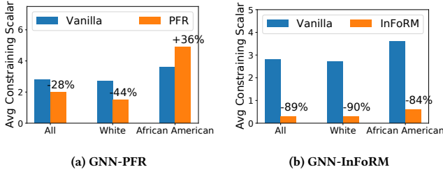
Figure 1: Average constraining scalar optimization based on PFR and InFoRM. Percentages denote the optimization results compared with vanilla values. Group disparity is exacerbated because the White group receives better optimization results compared with the group of African American.
